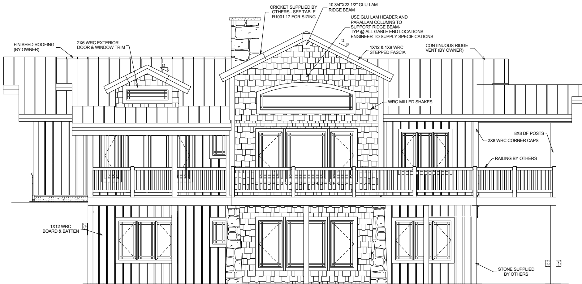
REAR ELEVATION
